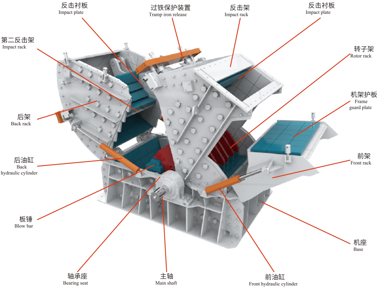
Structural Drawing
